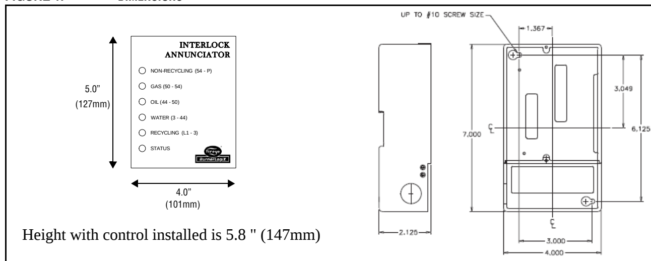
FIGURE 1. DIMENSIONS
