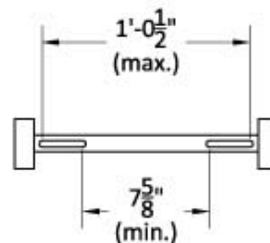
Spacer Bar Detail (Showing Range of Bolt Spacing)
