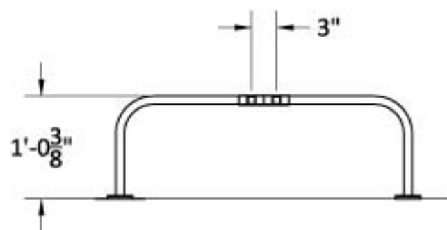
Side View - Retracted
