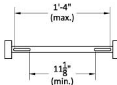
Spacer Bar Detail (Showing Range of Bolt Spacing)
