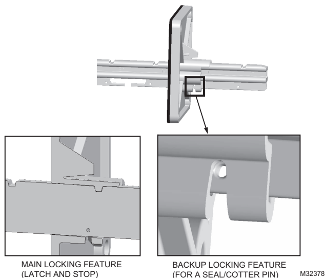
Fig. 6. Locking features.
