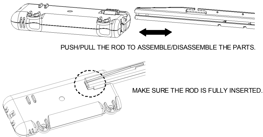
Fig. 2. Sensor attachment to rod.
