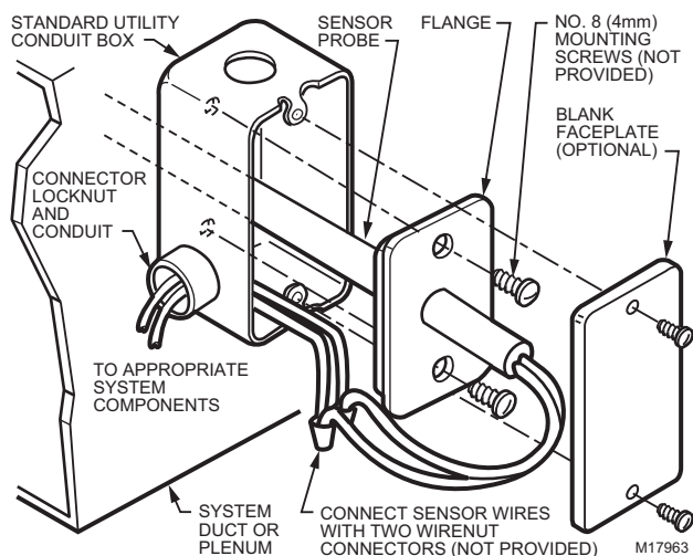
Fig. 3. Mounting C7770A/C7776A/C7778A Air Temperature Sensor in a standard conduit box.
