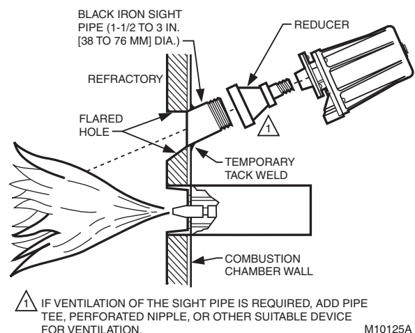
Fig. 5. Typical mounting of C7961.
