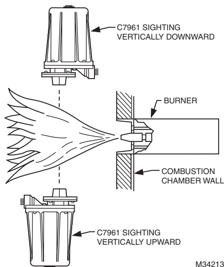
Fig. 6. Vertical mounting of C7961E.
