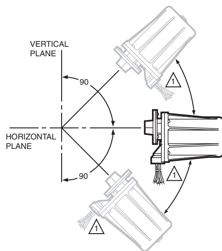
Fig. 6. Vertical mounting of C7961E.
