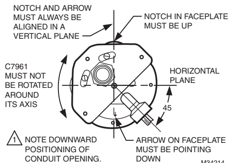
Fig. 7. C7961 mounting positions.
