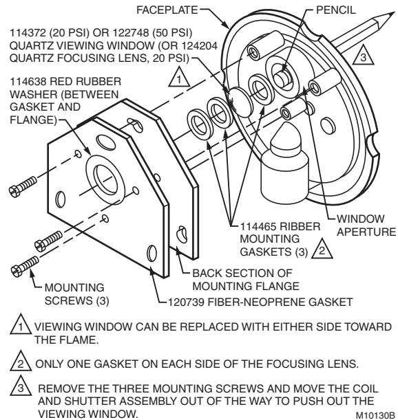
Fig. 12. Replacing quartz viewing window or focusing lens.
