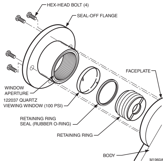
Fig. 13. Replacing quartz viewing window on C7961F.
