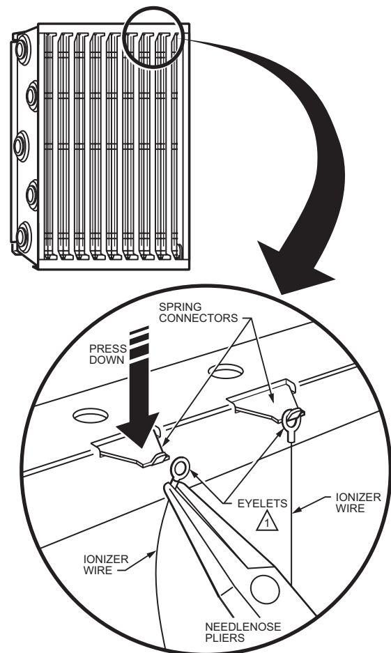
1 TWO EYELETS HOLD IONIZER WIRE TO CELL.
