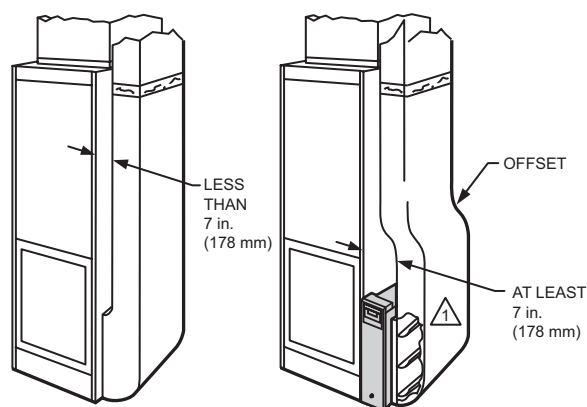
1 REQUIRED TURNING VANES HELP DISTRIBUTE AIRFLOW EVENLY. M948B
