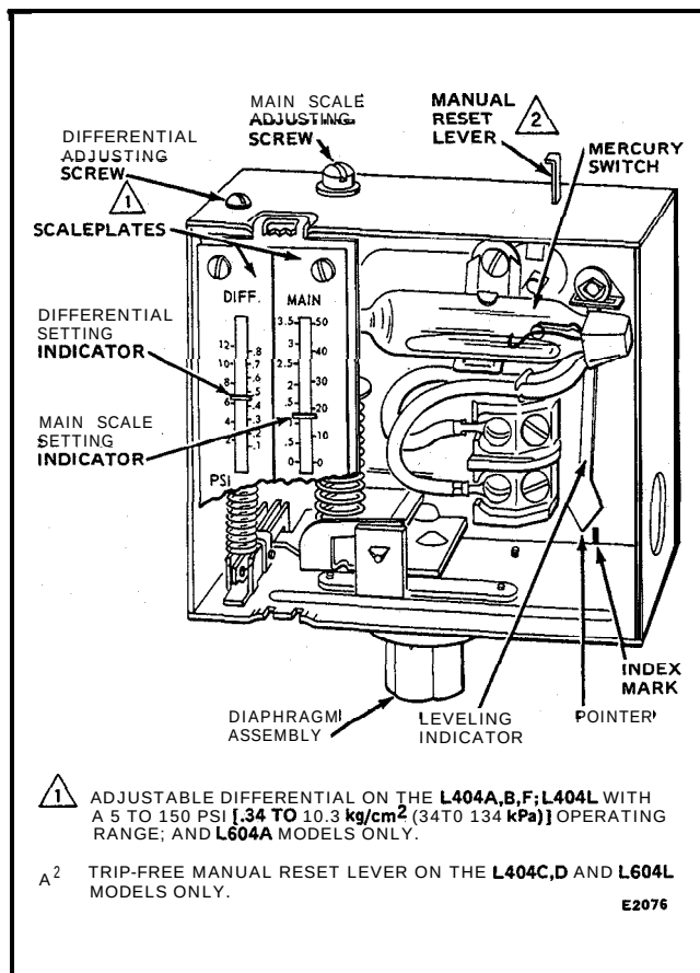
FIG. 1-SETTING A PRESSURETROL CONTROLLER.
