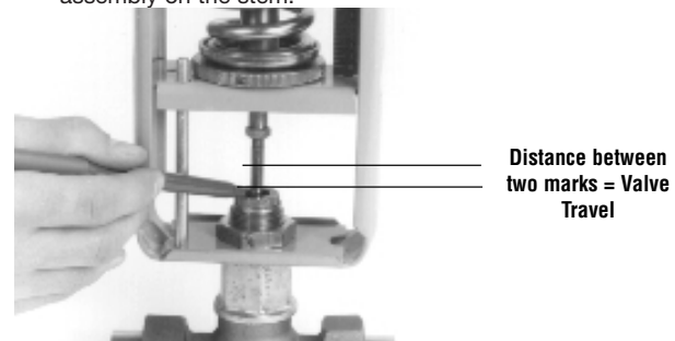
15. VALVE TRAVEL MEASUREMENT
