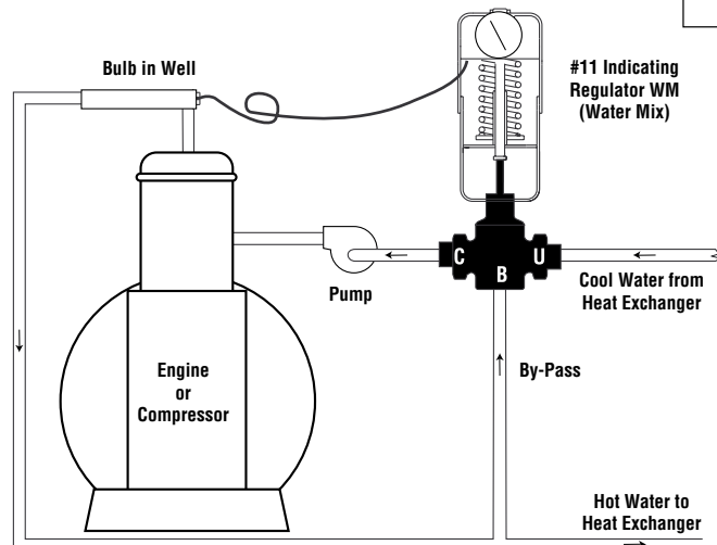
JACKET WATER COOLING APPLICATION
