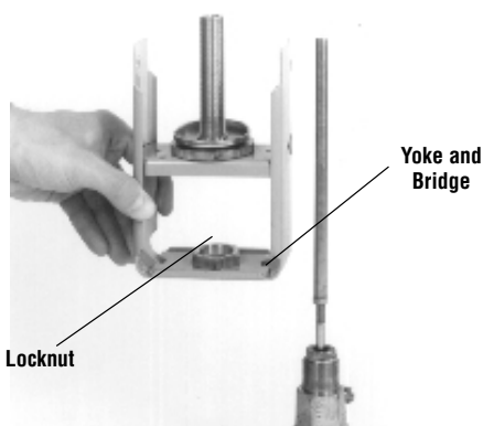
10A. (1/2" TO 2") LIFT OFF BRIDGE/YOKE ASSEMBLY
