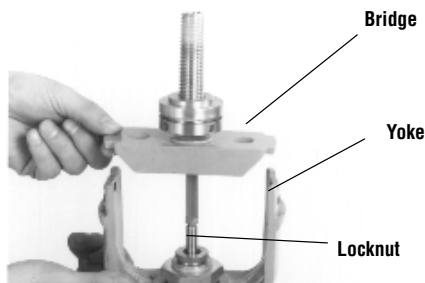
10B. (2-1/2" TO 4") LIFT OFF BRIDGE AND YOKE
