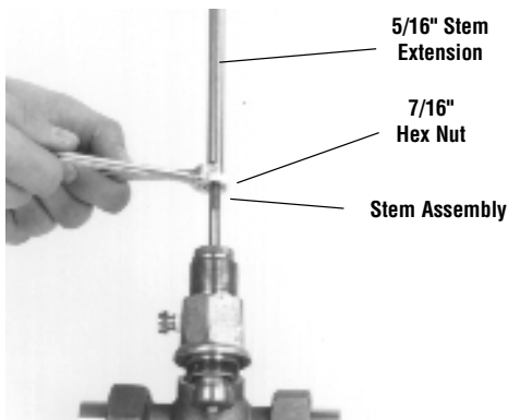
11. REMOVE STEM EXTENSION AND HEX NUT
