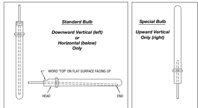
5A. BULB ORIENTATION
