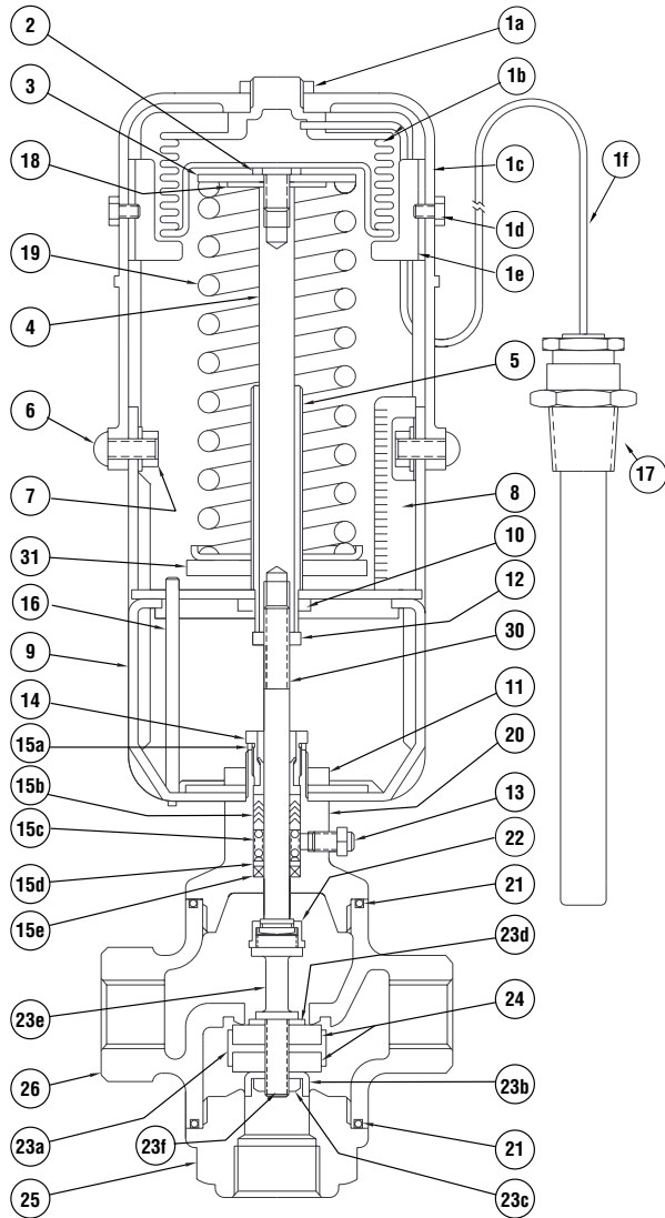
1/2" - 2" WM Assemblies
