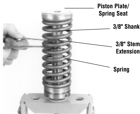
9B. (2-1/2" TO 4") REMOVE PISTON PLATE/SHANK AND SPRING
