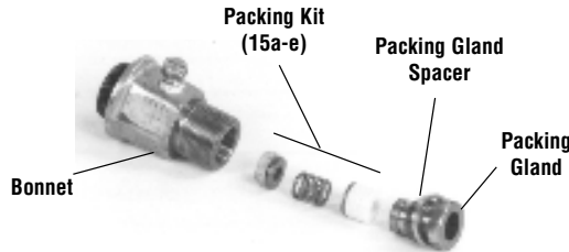
13. PACKING COMPONENTS
