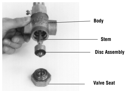
12A. (1/2" TO 2") PLUG ASSEMBLY
