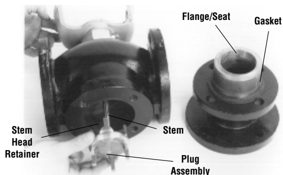
12B. (2-1/2" TO 4") PLUG ASSEMBLY
