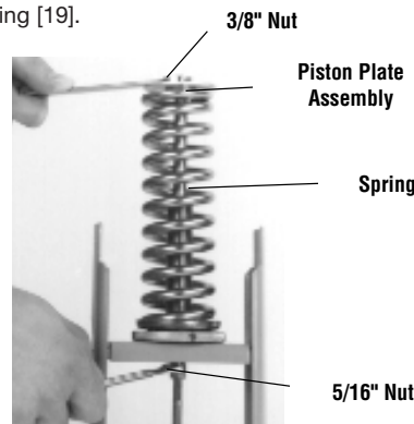
9A. (1/2" TO 2") REMOVE PISTON PLATE AND SPRING
