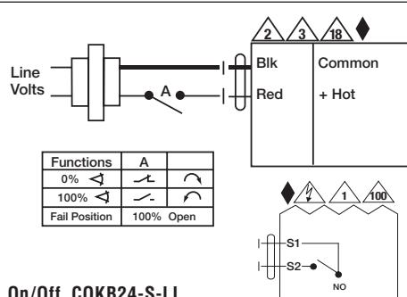
On/Off, CQKB24-S-LL
