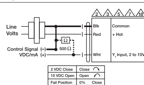
Proportional, CQKB24-SR-LL
