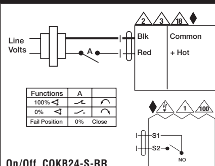
On/Off, CQKB24-S-RR
