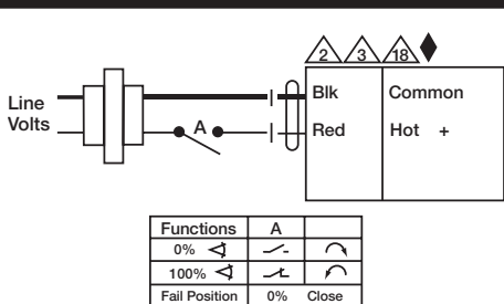
On/Off, CQKB24-RR
