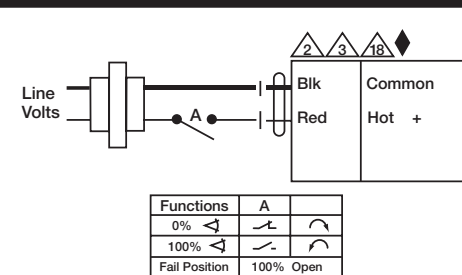
On/Off, CQKB24-LL
