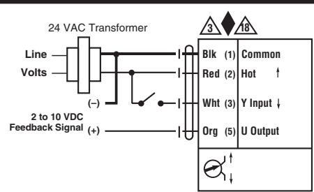
Triac Sink
