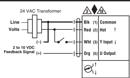
Triac Sink
