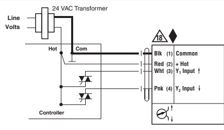
Triac Source
