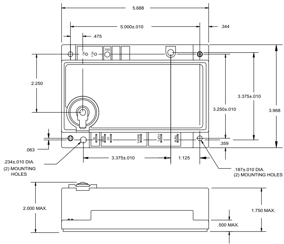
Figure 4. Standard Enclosure
