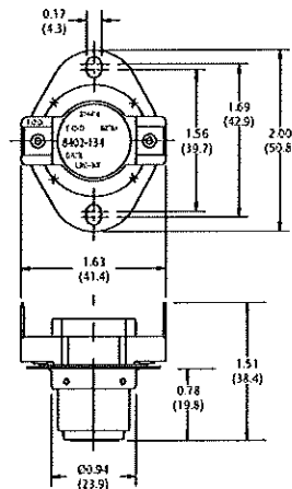
SPST Airstream Mounting – Deep Disc Cup
