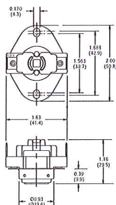
SPST Manual Reset – Airstream Mounting
