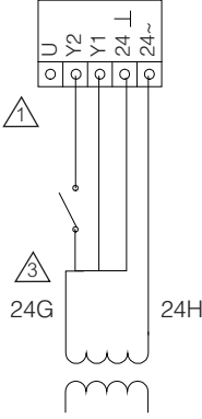
24 VAC Two Position Sinking
