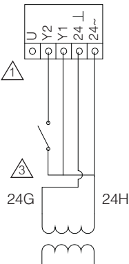
24 VAC Two Position Sourcing
