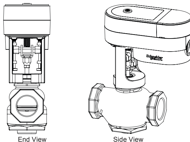
MG350V Installed on a VB-7000 Globe Valve
