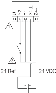
24 VDC Two Position Sourcing
