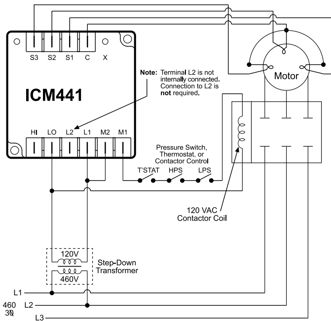
Step-Down Transformer Powering ICM441 and Contactor
