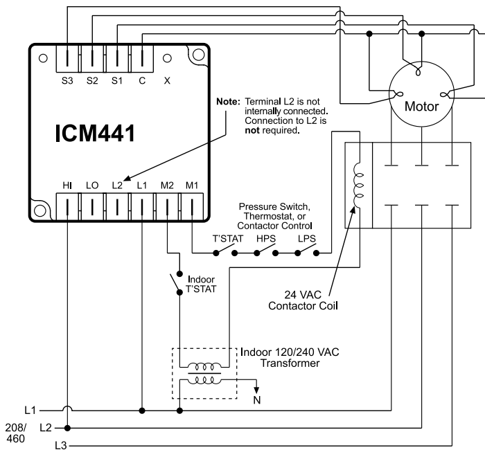
Step-Down Transformer Powering ICM441 and Contactor
