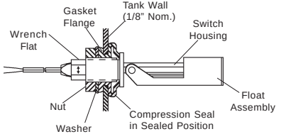
LS-7 with Compression Seal (Type 10)
