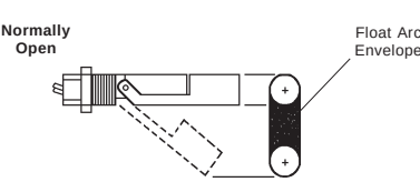
The switch is mounted so that the float lowers with the liquid level. The switch is N.O.
