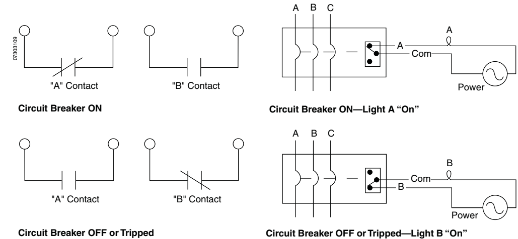
Figure 6: Auxiliary Switch Wiring Diagrams
