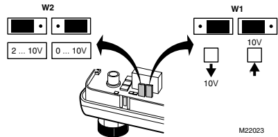
Fig. 7. Switch selection according to controller output signal and valve type (two-way or three-way).
