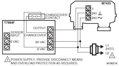
Fig. 6. M7435F used with T7984F.
