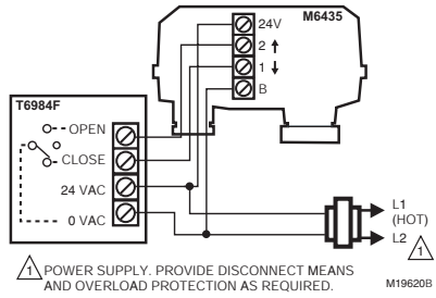
Fig. 5. M6435A used with T6984F.
