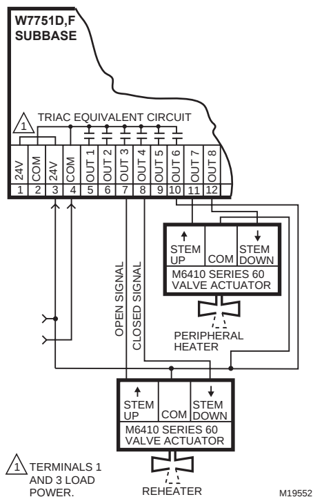
Fig. 11. M6410A Actuator wired with W7751D,F Controller.
