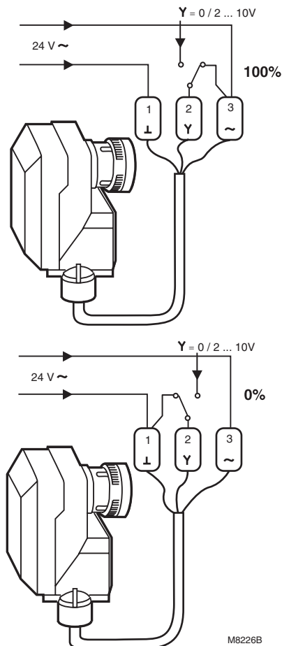
Fig. 14. Input signal override for frost protection.
