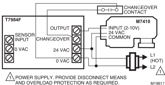
Fig. 9. M7410F used with T7984F.
