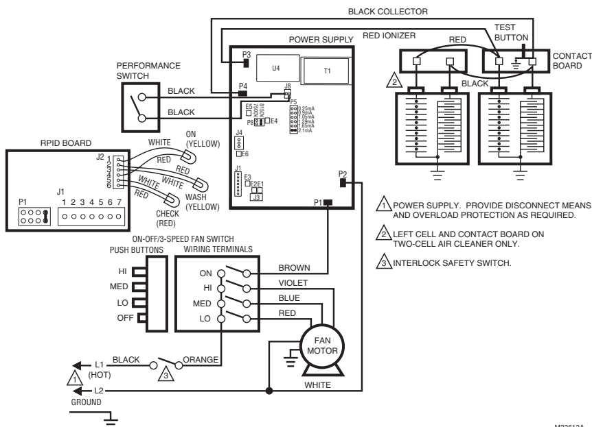
Fig. 19. Recent F90 schematic diagram.
