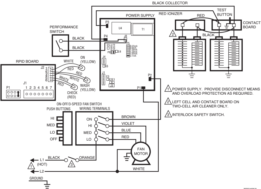
Fig. 13. Recent F57 120V model electrical schematic.
