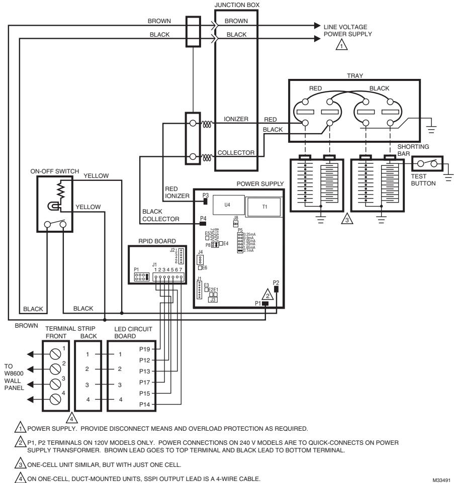
Fig. 7. Past electronic air cleaner (F50A&E, F52E) with W8600E—internal schematic.
