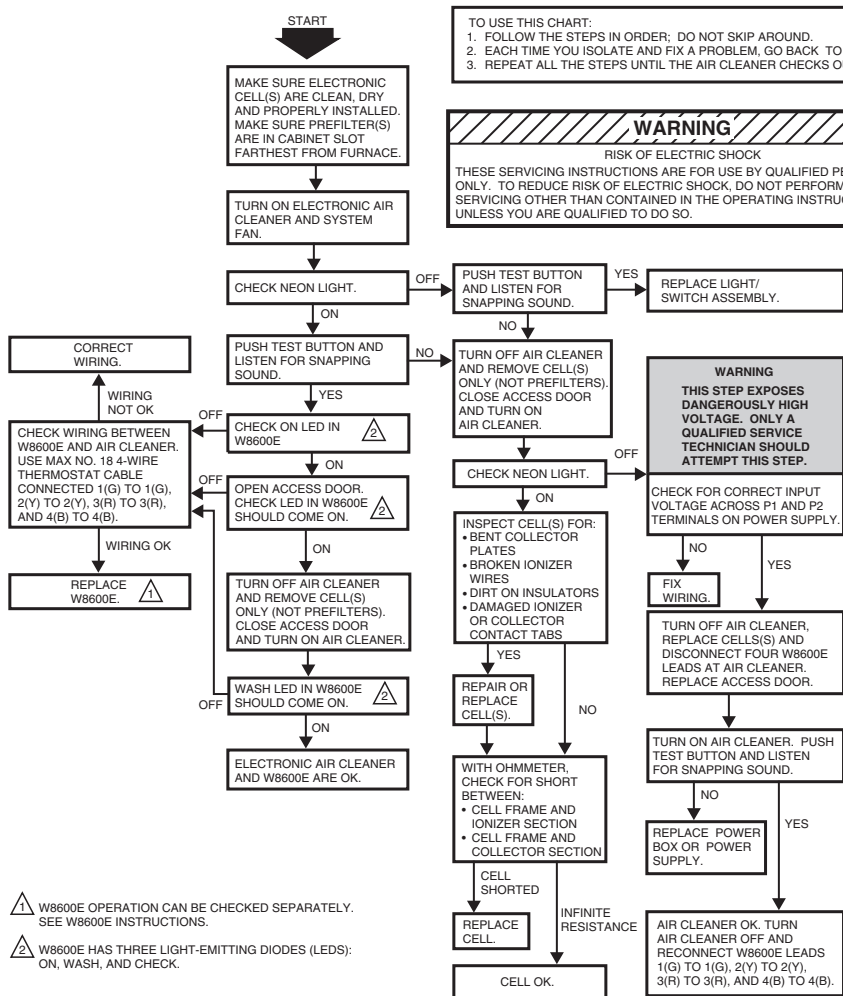
Fig. 21. Troubleshooting air cleaners with solid-state performance indicator.
