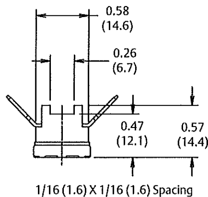
TM, TMH, TME Surface Mount
