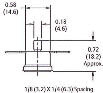
TX Surface Mount
