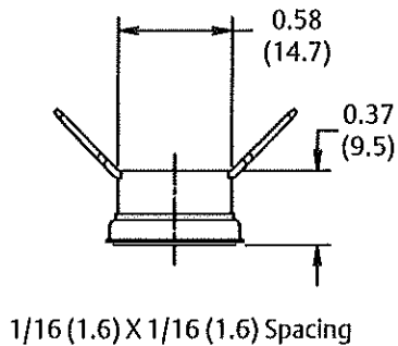
T, TE, TH Surface Mount
