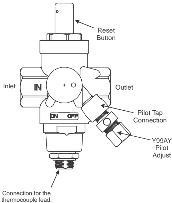
Figure 3: Typical H19 Valve with Rotor Valve
