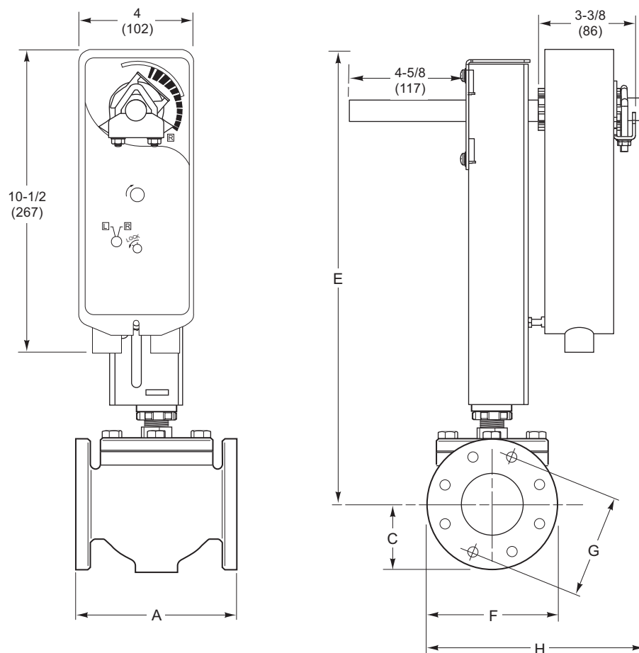
Figure-32 Mx41-715x-2xx or Mx41-707x-2xx with 2-1/2" to 4" 2-Way Flanged Globe Valve with AV-607-1 Linkage.
