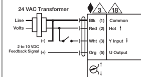
Non-Spring Return Actuator with MFT
