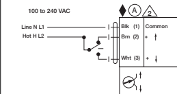
Floating Point
