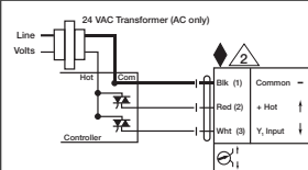
Triac Source
