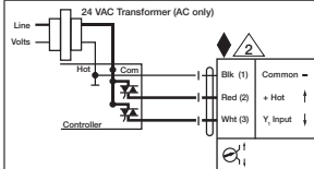
Triac Sink
