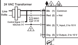
Non-Spring Return Actuator with -SR
