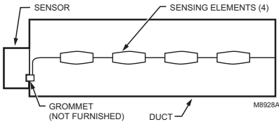
Fig. 3. Duct cross section showing method of installing C7021J, C7023J/C7031J/C7041J in a multizone system.
