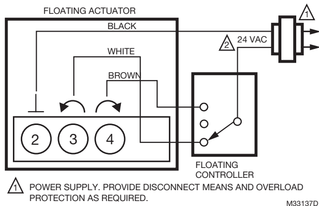
Fig. 16. MVN613 with Floating Control.
