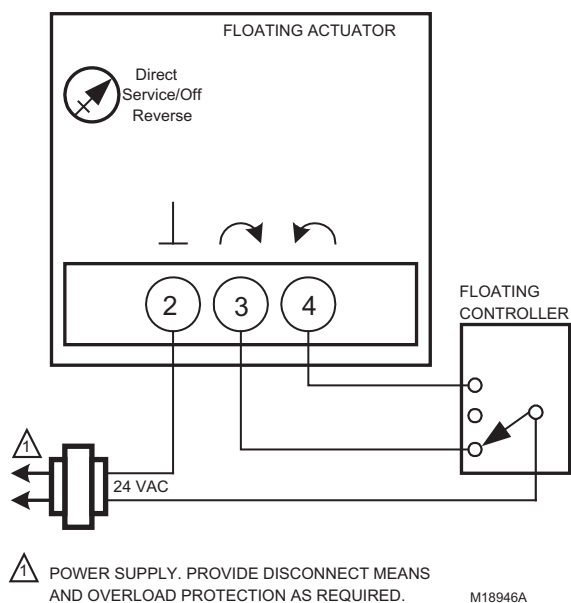
Fig. 13. MN6105 with Floating Control.
