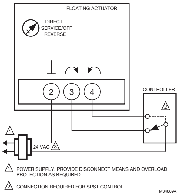
Fig. 12. MN6105 with On/Off SPDT Control.
