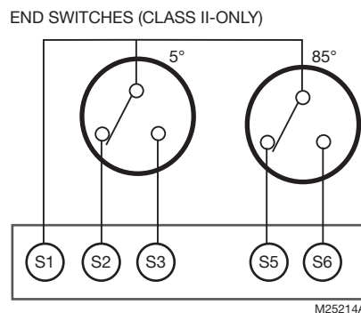
Fig. 15. Wiring for MN6105 and MN7505 models with aux./end switches.
