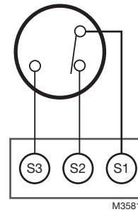
Fig. 20. Wiring for model with aux./end switches.
