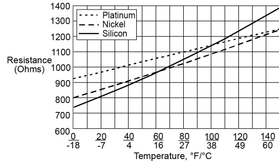
Figure 2: Nickel, platinum, and silicon temperature response
