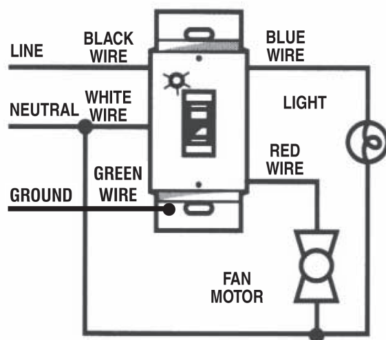
FAN/LIGHT WIRING
