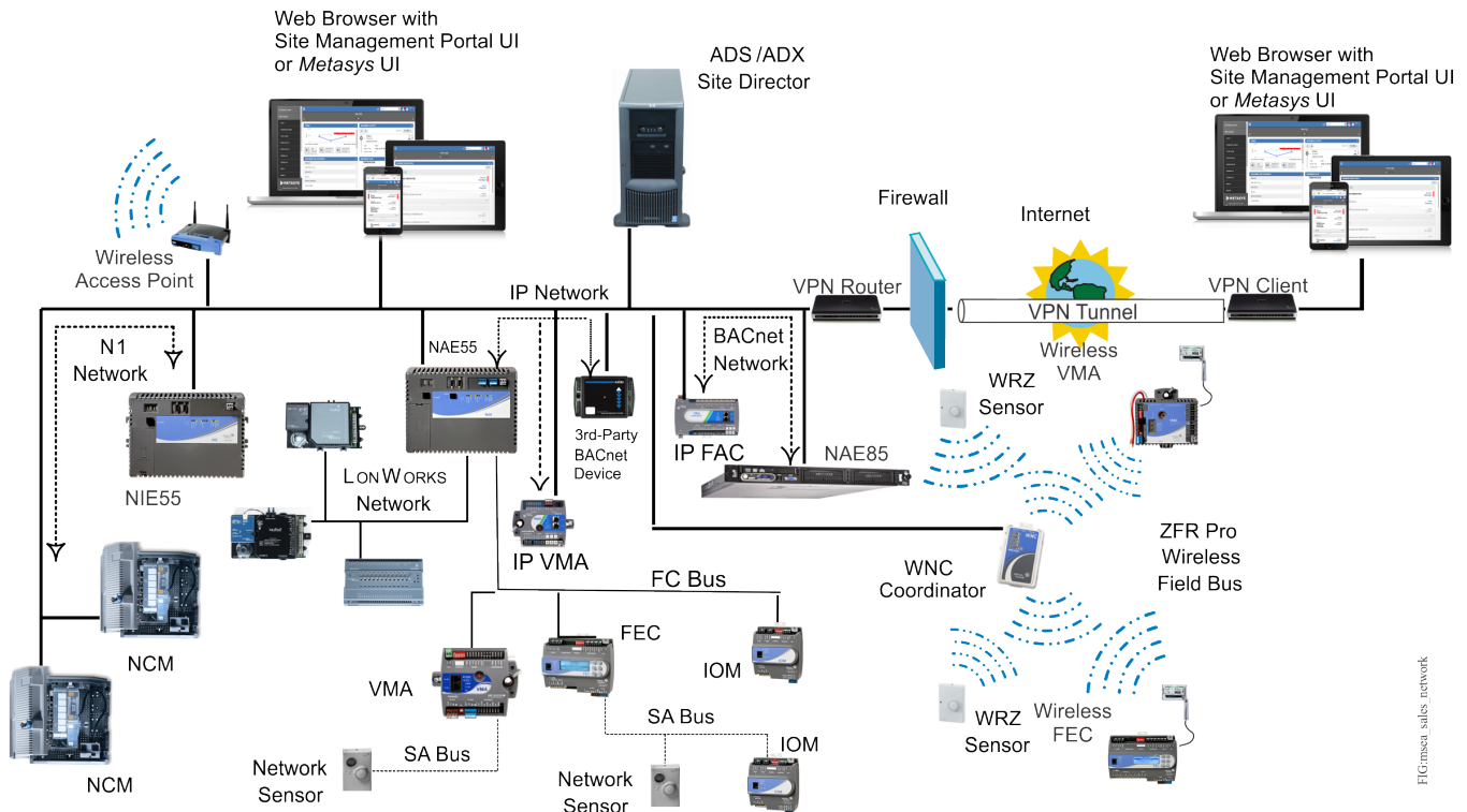
Figure 2: Metasys System with Field Equipment Controllers
