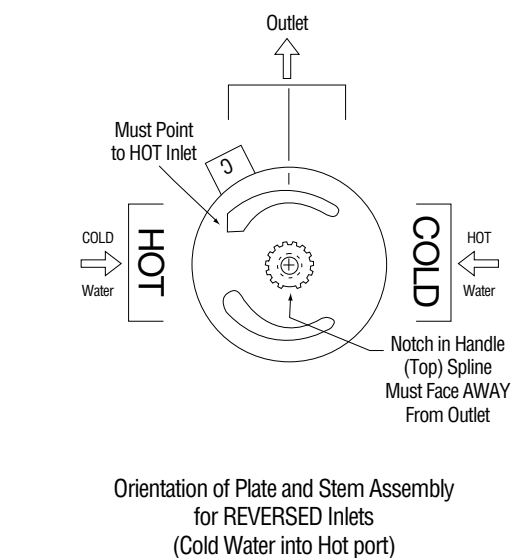
FIGURE 3 – REVERSED INLETS
