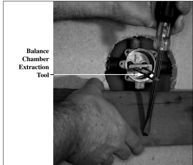
FIGURE 4 – BALANCE CHAMBER REMOVAL
