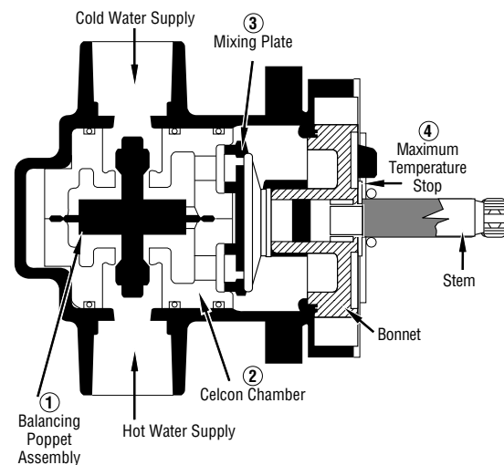
FIGURE 1 – OPERATION
