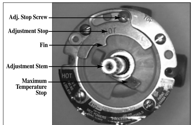
FIGURE 5 – MAXIMUM TEMPERATURE SETTING
