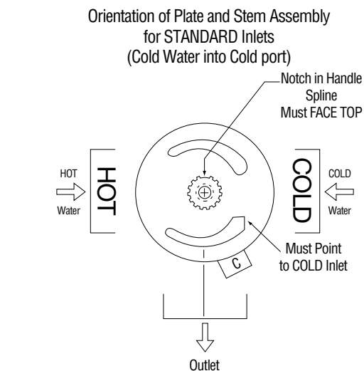
FIGURE 2 – STANDARD INLETS
