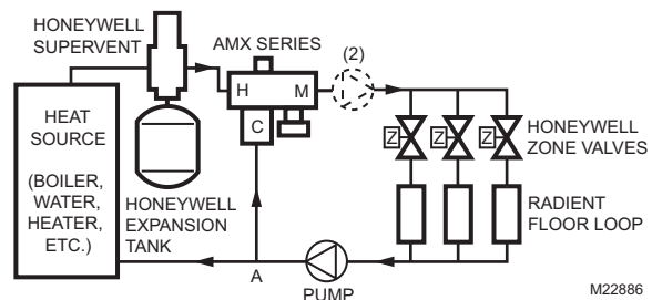
Fig. 4. Single Loop.
