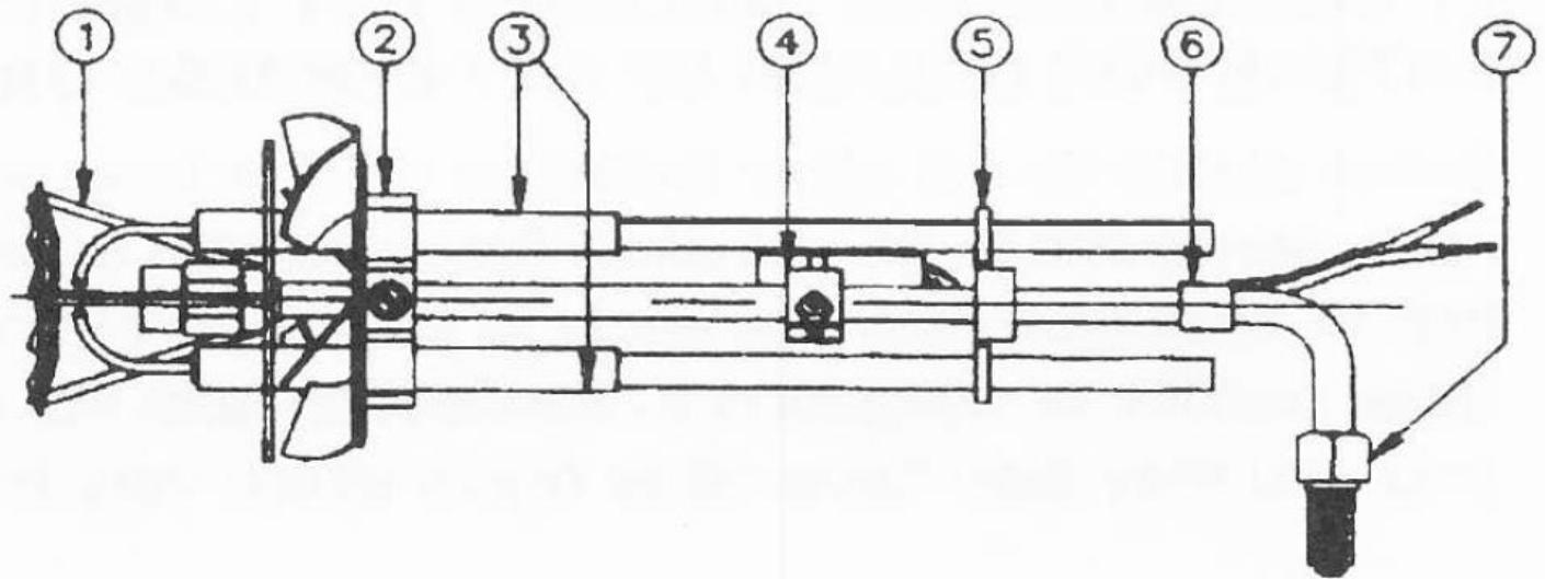
Figure 2– Oil Gun Assembly Detail View
