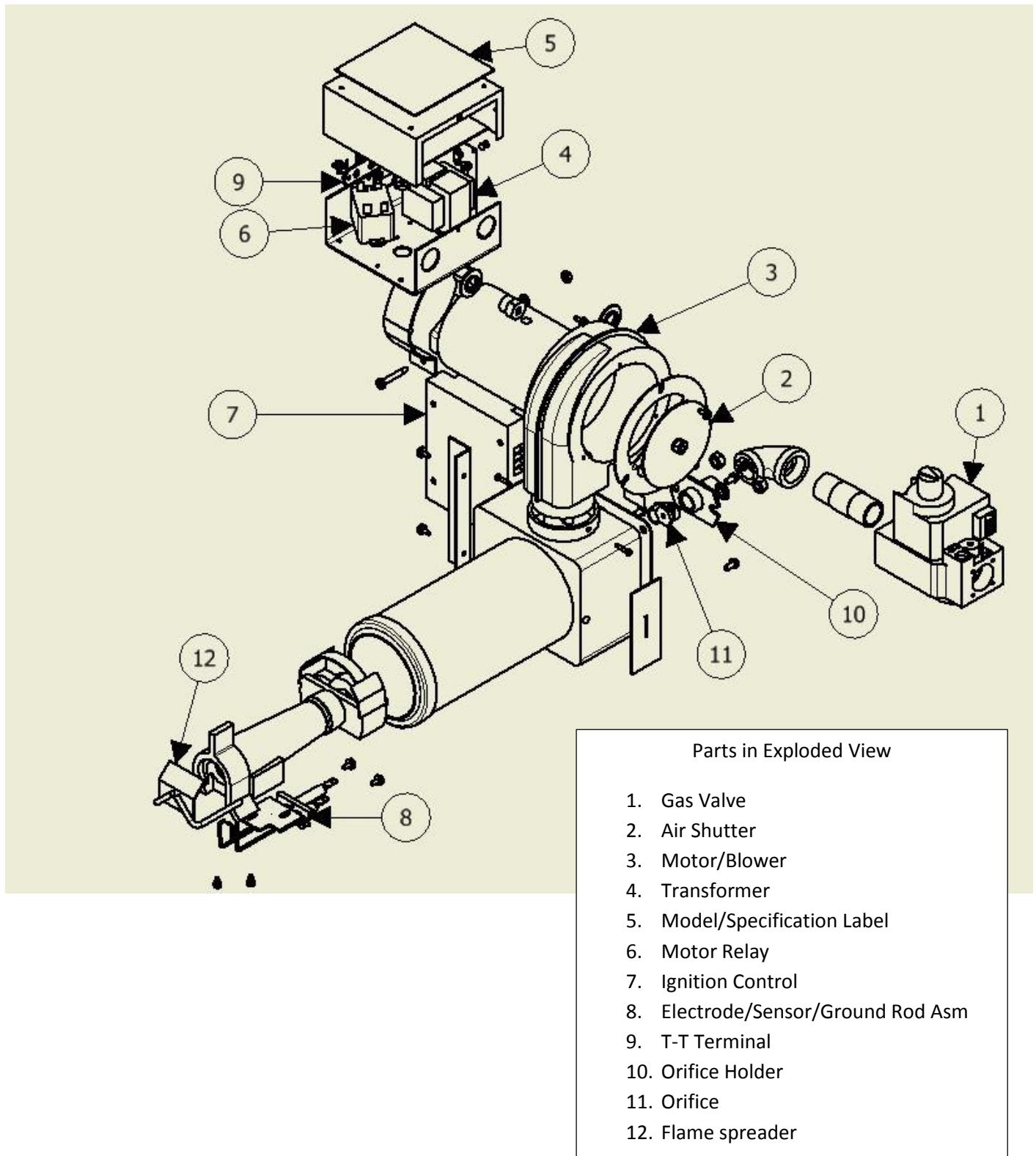
FIGURE 27: Right Side Exploded View of P265F
