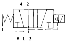
4-Way 2 position solenoid external pilot
