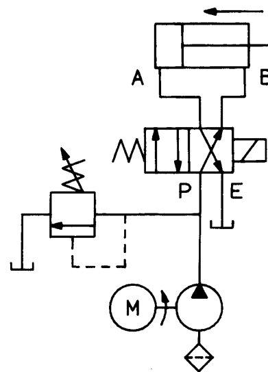
Energized
