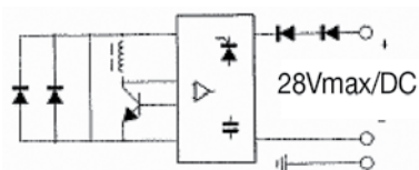
Wiring Schematic for Booster Circuit
