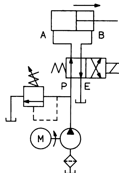
De-Energized
