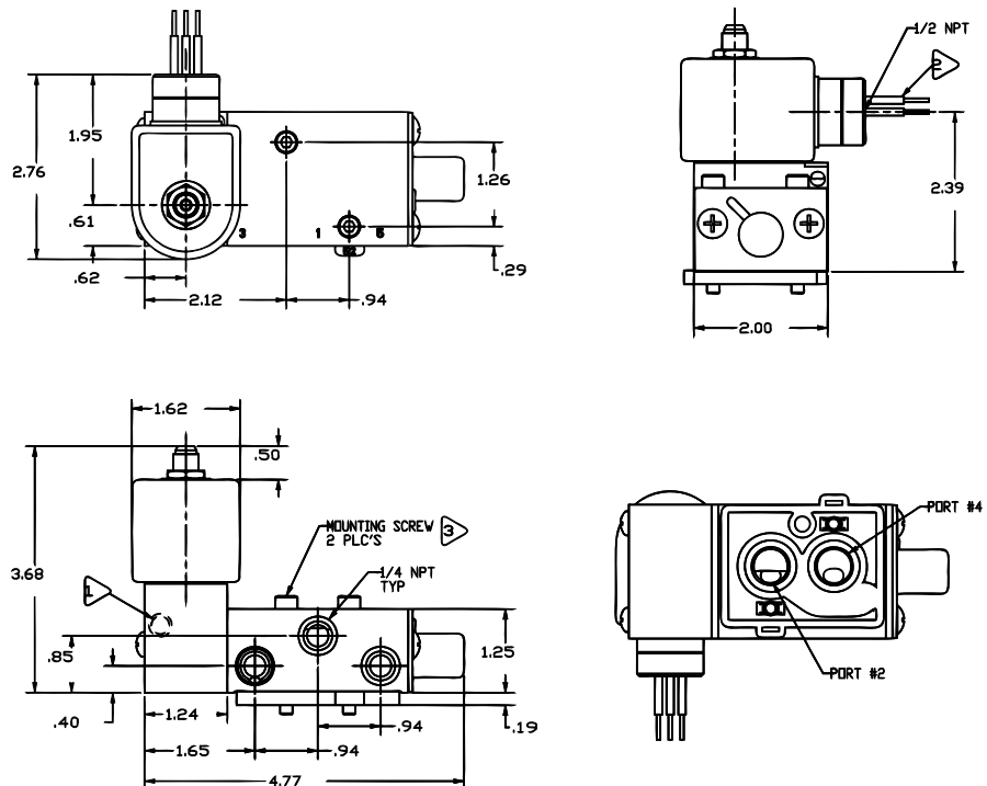
5/2, 4-Way 2 Position Single Solenoid
