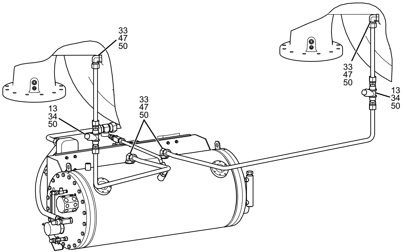
1" Piping J1-J5, K1-K4 and K7 Compressors
