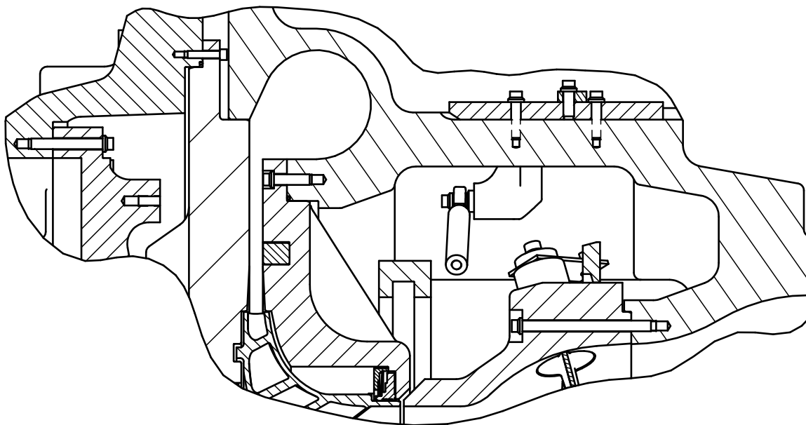
SECTION J-J
