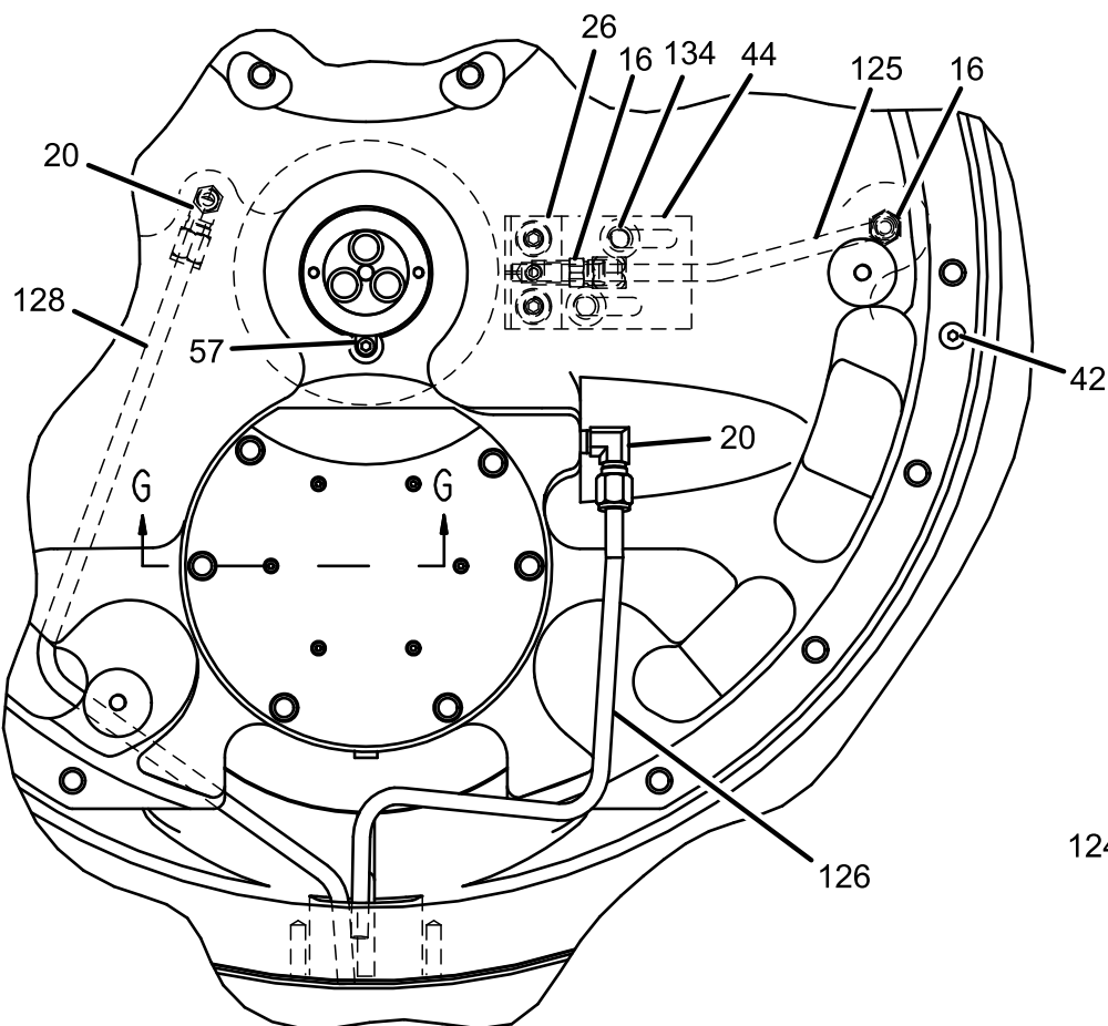
SECTION B-B
